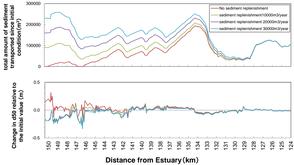
Fig. 6: Simulation results of the average grain size (d50), sediment transport volume and riverbed material due to changes in sediment replenishment volumes
